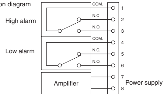
Connection diagram
